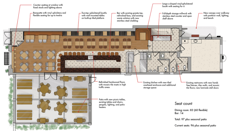
Shamrock Pub | Floor Plan ptd patrick thompson design, inc. www.patrickthompsondesign.com
